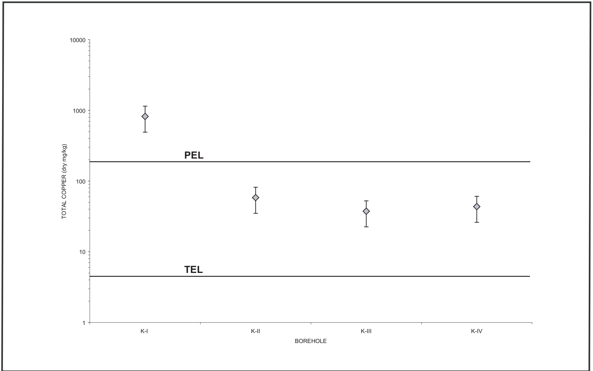
Figure 5 Kilarc Diversion Dam Total Cu Results By Borehole Showing 40% Margin of Error, TEL, and PEL Thresholds
