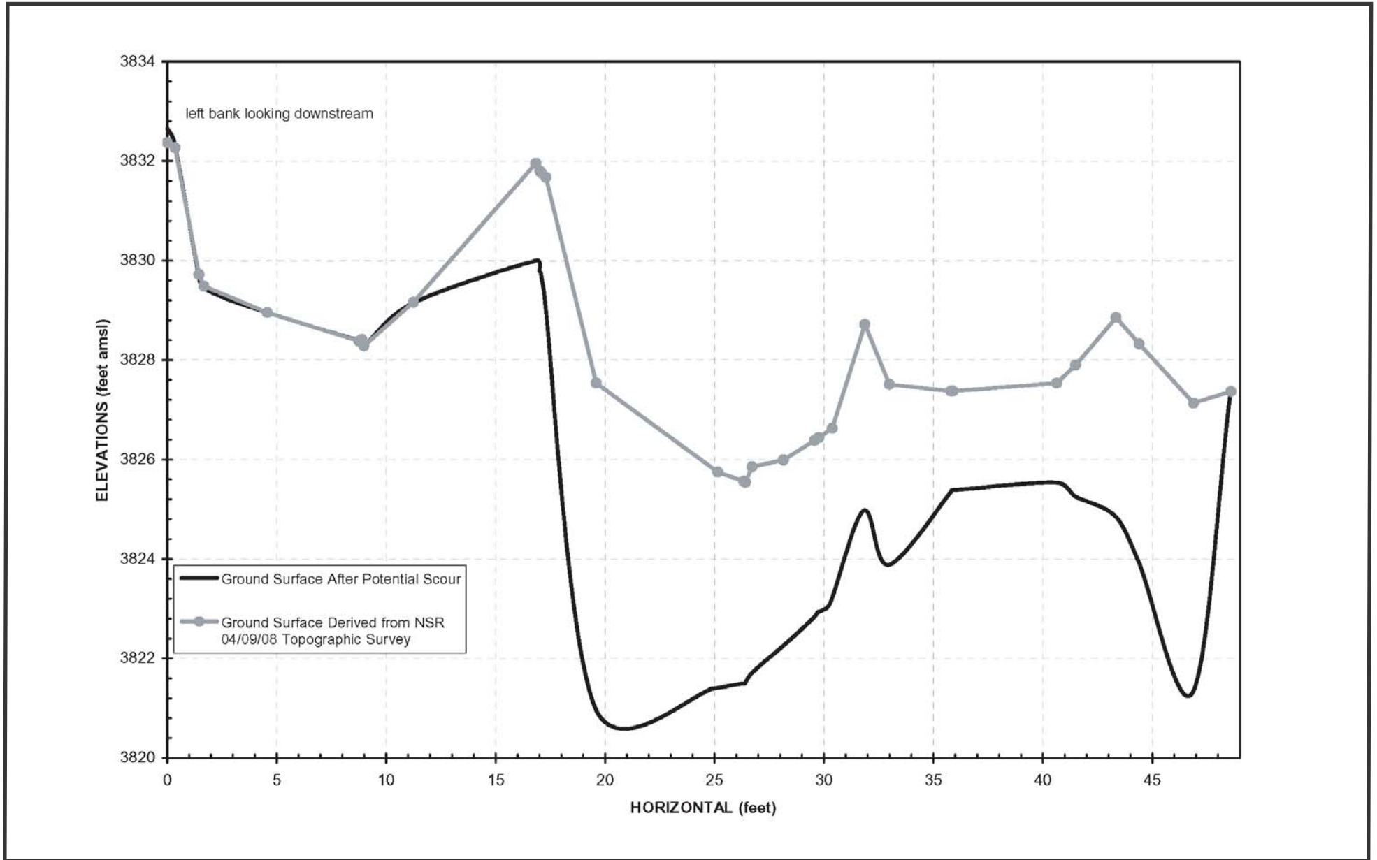
Figure 9 Stream Channel Cross-Section X-2 Showing the Present Bed Elevation and Potential Elevation After Scour Thalweg is likely to migrate north along exposed bedrock and boulder material that forms the right bank at this cross-section.
