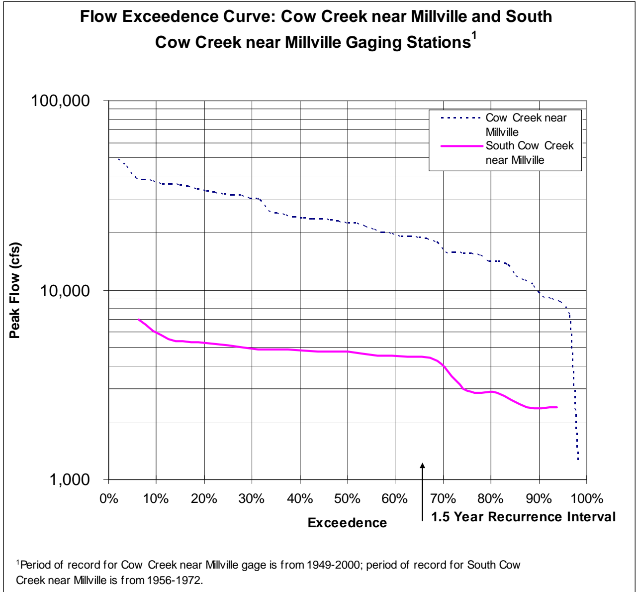
Figure 1. Flood Frequency Curves for Cow Creek near Millville (gage No. 11374000) and South Cow Creek near Millville (gage No. 11372200).
