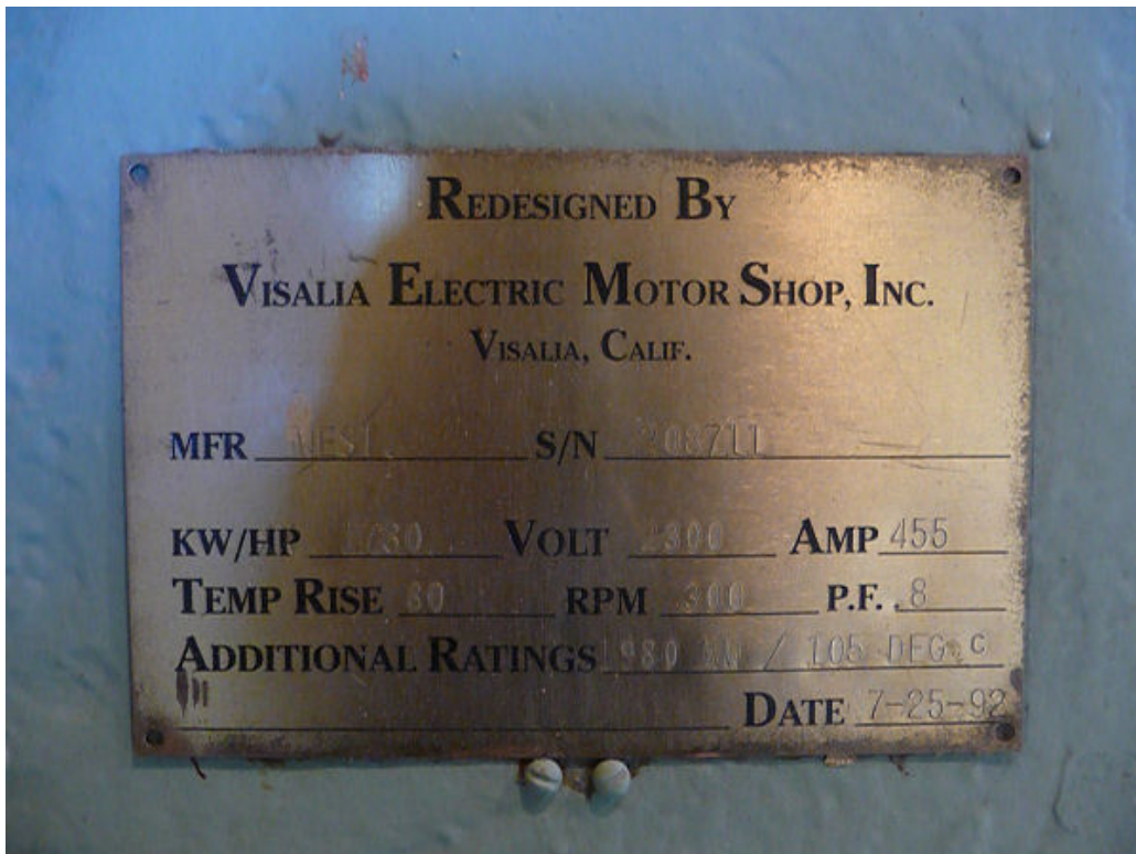
Picture 2 – Kilarc Rebuild Plate
